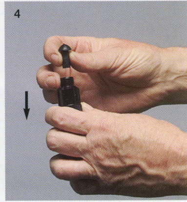
4 Set mushroom plug into Plugger with stem down
