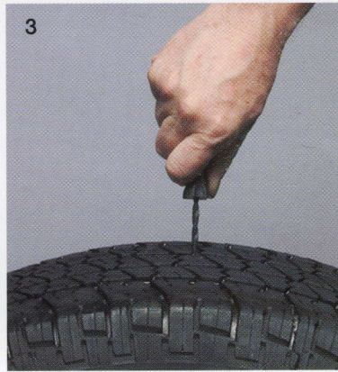
3 Thoroughly ream out hole with rasp tool
