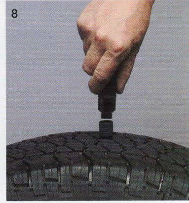
8 Screw loaded Plugger onto nozzle in tire
