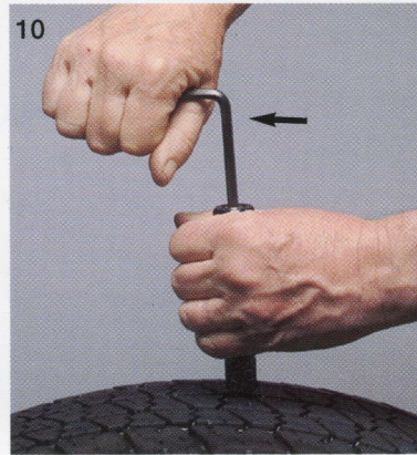
10 Then turn counter-clockwise until inner rod returns to bottom of Plugger
